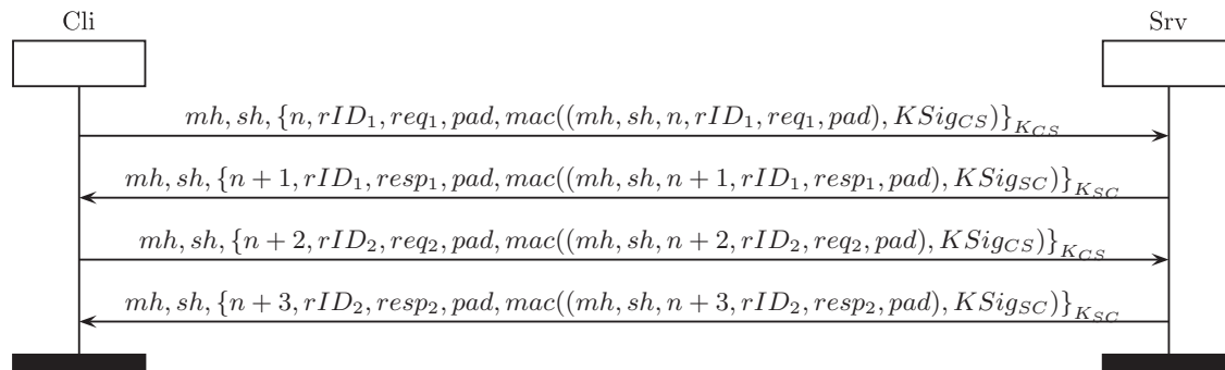
Fig. 5 – Two requests and responses in OPC-UA.
