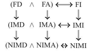
Fig. 1 – Relationship of our notions: A \Rightarrow B if a protocol ensuring A also ensures B .
