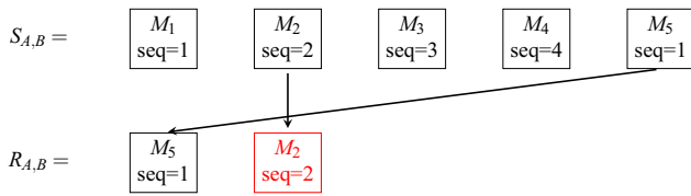
Fig. 6 – Message reordering attack example.
