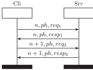
Fig. 2 – Two requests and responses in textbook MODBUS (MODBUS, 2004).
