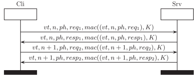
Fig. 4 – Two requests and responses in secure MODBUS (Hayes and El-Khatib, 2013).
