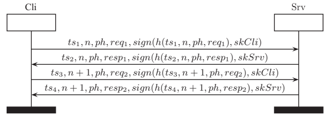
Fig. 3 – Two requests and responses in secure MODBUS (Fovino et al., 2009).
