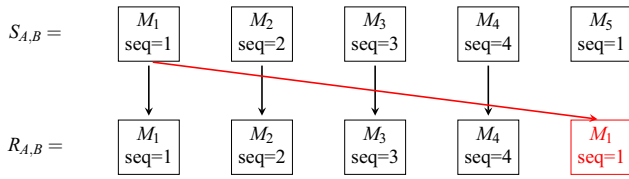
Fig. 7 – Message replaying attack example.
