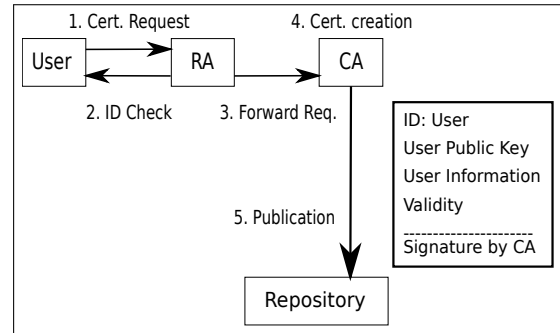
Figure 2: PKIX registration.
