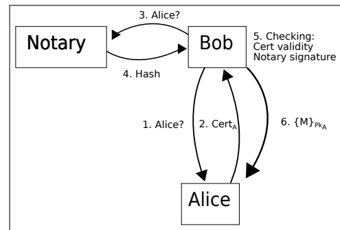
Figure 3: LOCALPKI end entity interactive authentication.
