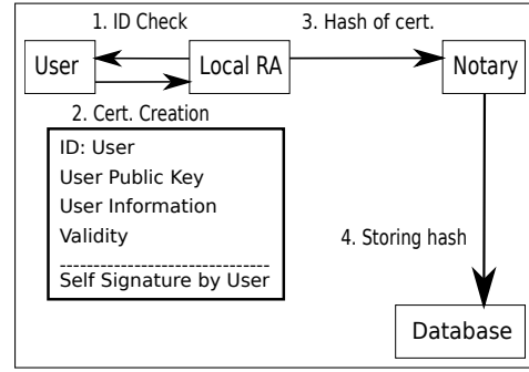
Figure 1: LOCALPKI registration.
